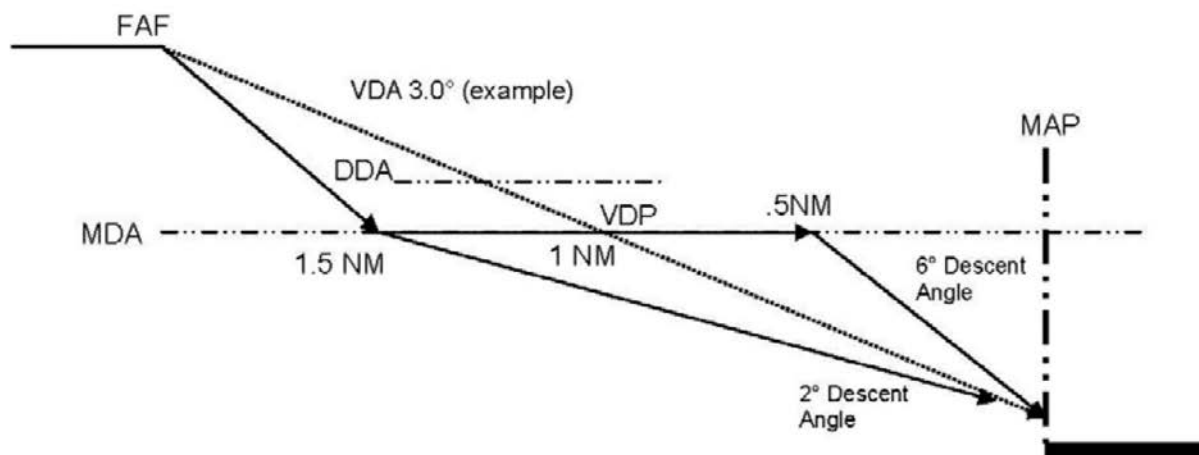
Figure 16.4. Dive and Drive.
