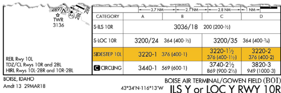
Figure 18.5. Published Side-Step Minimums.
