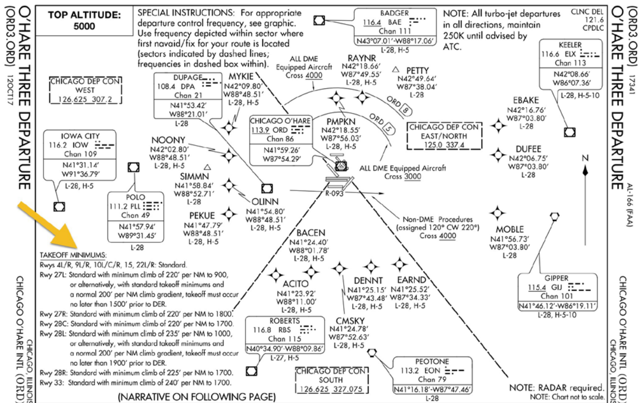
Figure 5.21. Civil SID.
