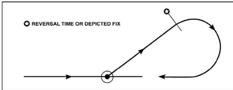
Figure 15.23. Base Turn or (NAS only) Teardrop.
