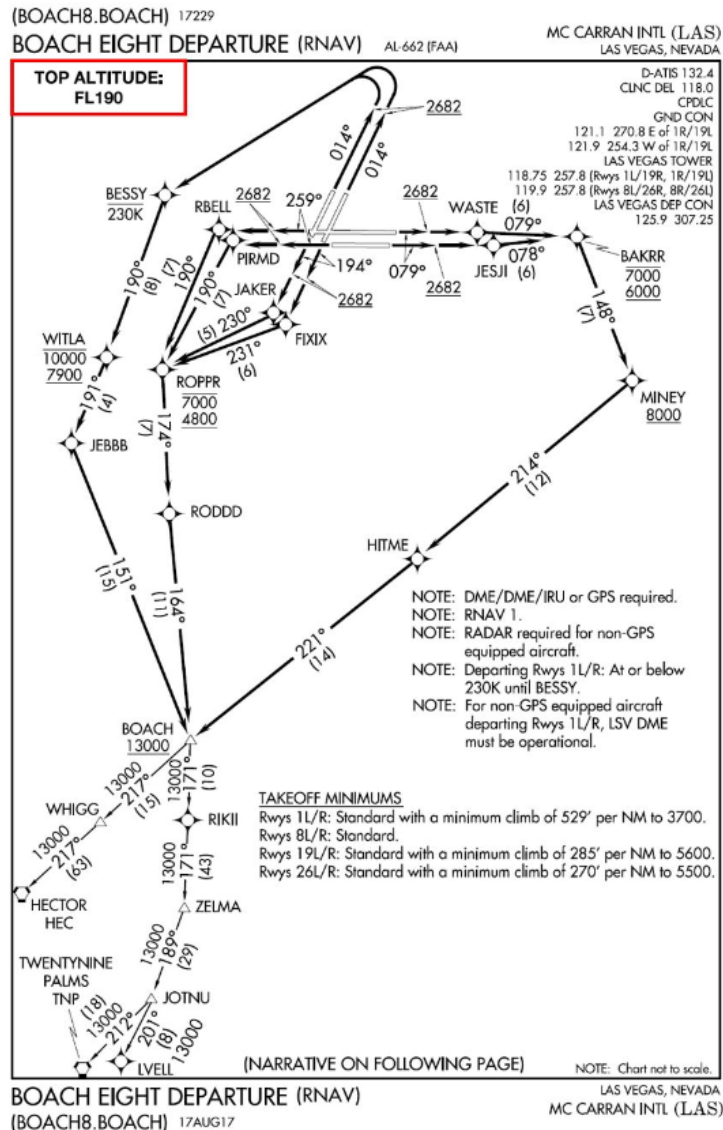
Figure 5.19. Civil SID with Top Altitude.
