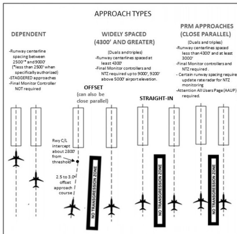
Figure 15.35. Simultaneous Approaches to Parallel Runways.
