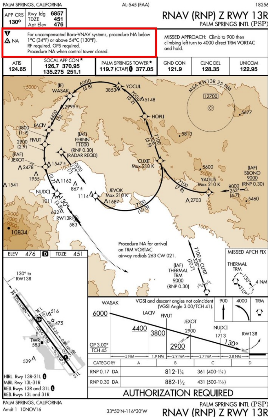
Figure 17.7. Nonstandard Missed Approach Climb Gradient.
