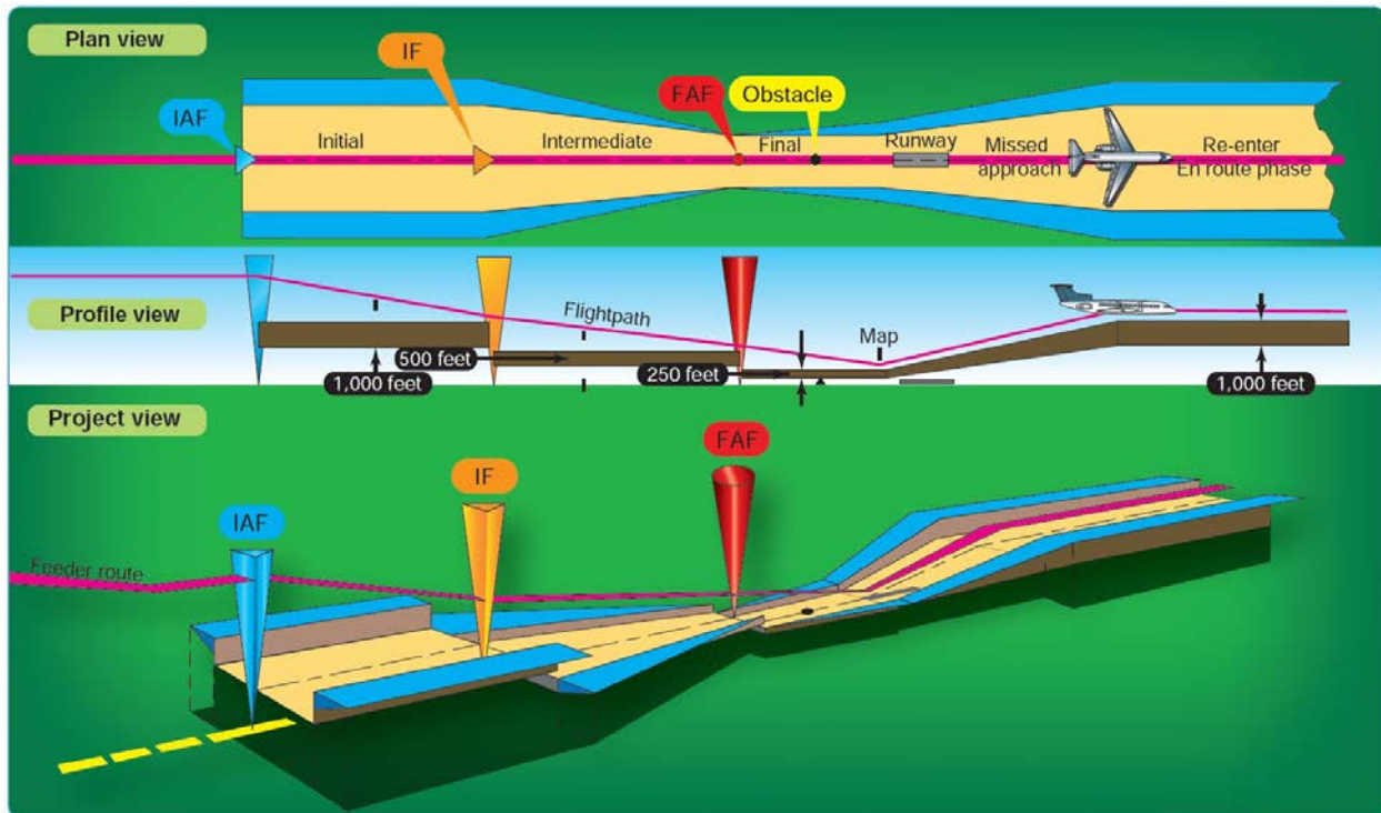
Figure 15.10. Approach Segments.
