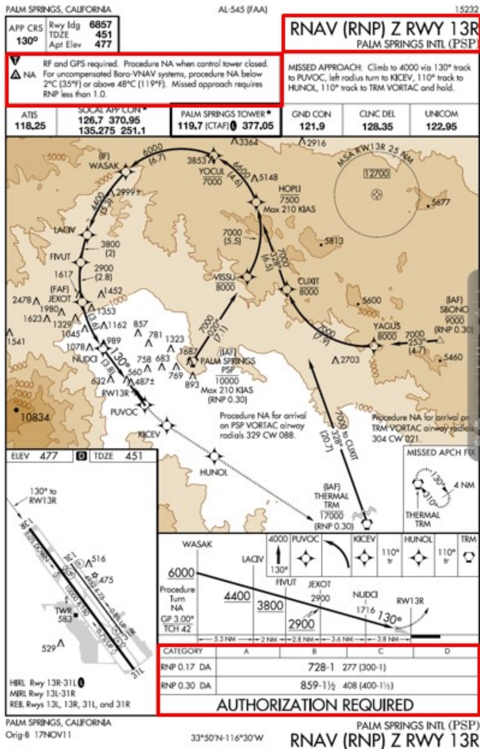
Figure 17.6. RNP Values.
