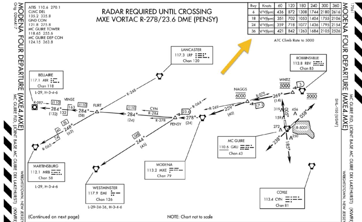
Figure 5.20. Military SID.
