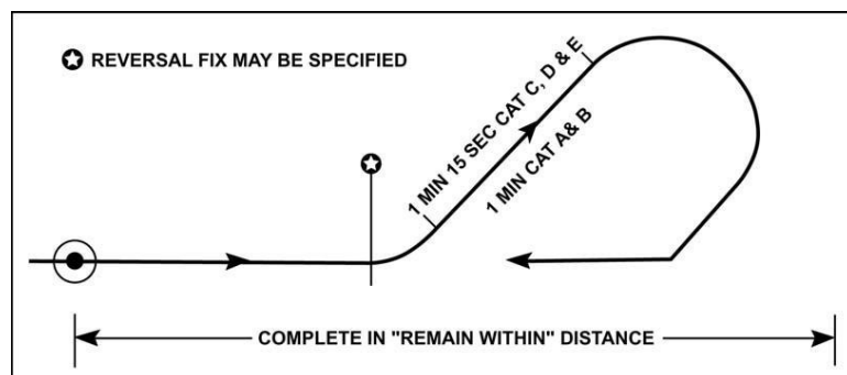
Figure 15.21. 45°/180° Procedure Turn.
