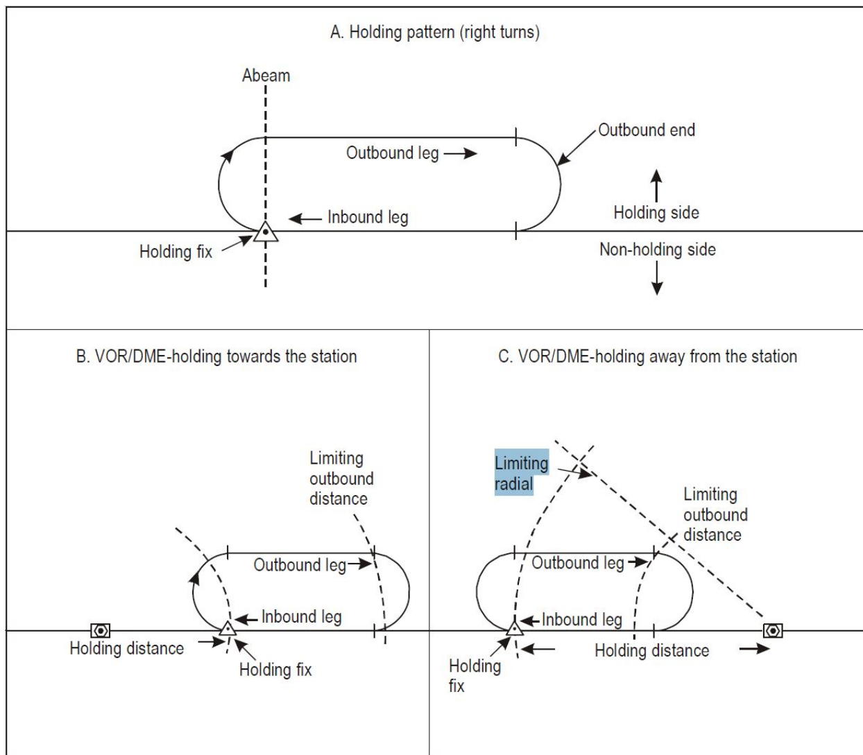
Figure 13.5. ICAO Limiting Radial.
