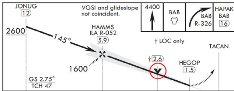
Figure 16.1. VDP.
