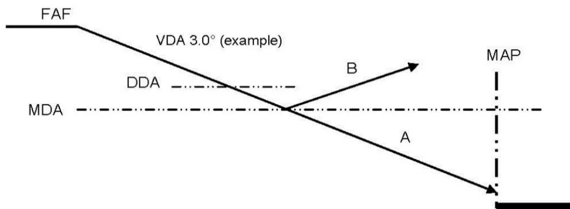
Figure 16.5. CDFA.
