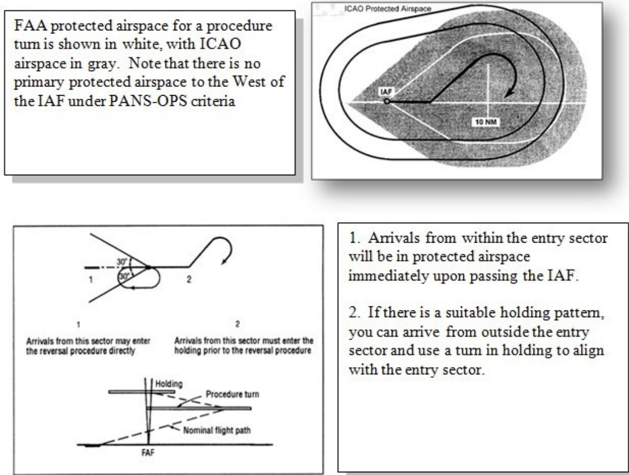
Figure 15.16. ICAO PANS-OPS versus U S TERPS Protected Airspace.
