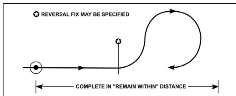
Figure 15.22. 80°/260° Procedure Turn.
