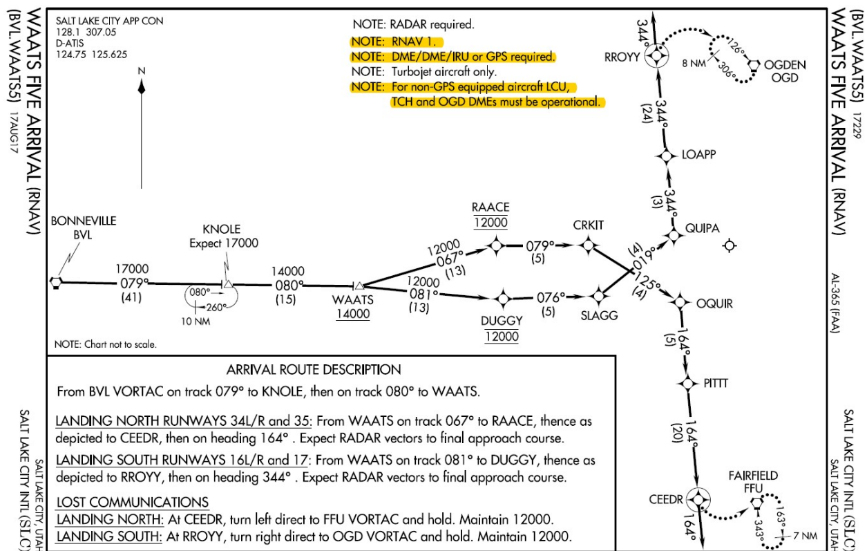
Figure 14.1. RNAV Arrival.
