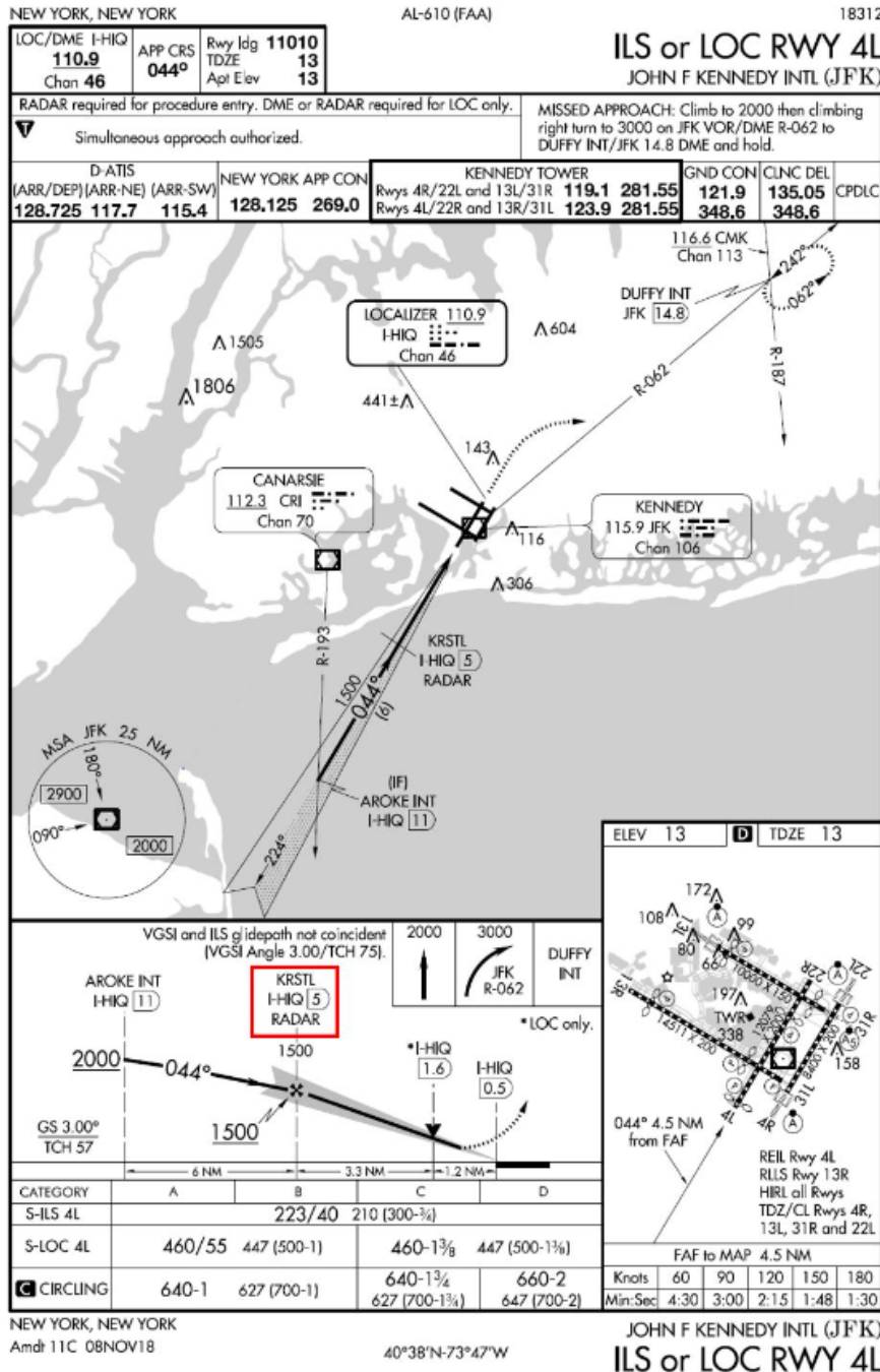
Figure 15.6. Radar Fix on Non-radar Approach.
