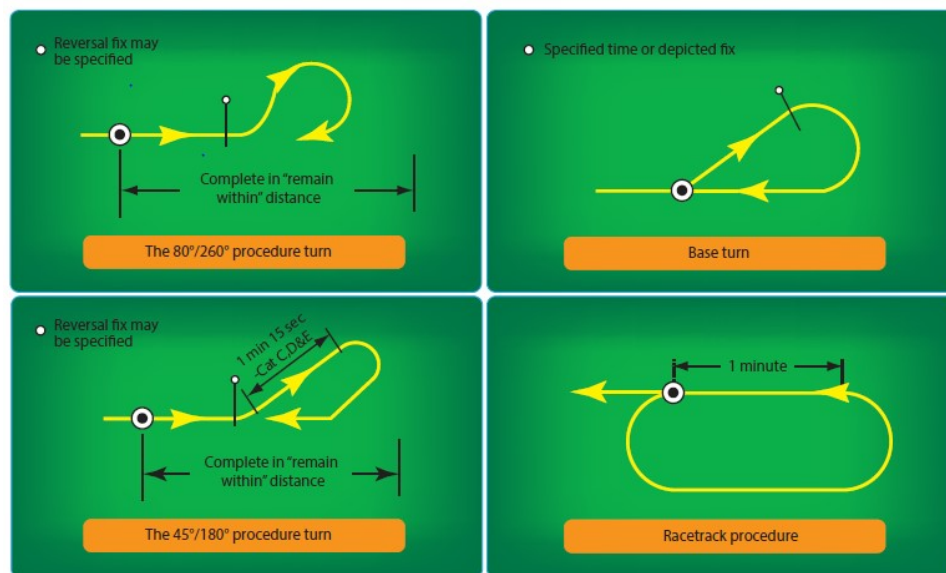
Figure 15.13. Types of Course Reversals.
