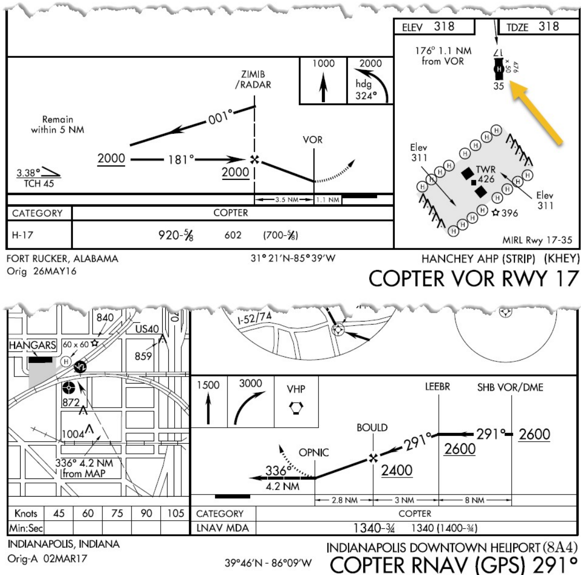
Figure 15.30. Helicopter-Only Approach.
