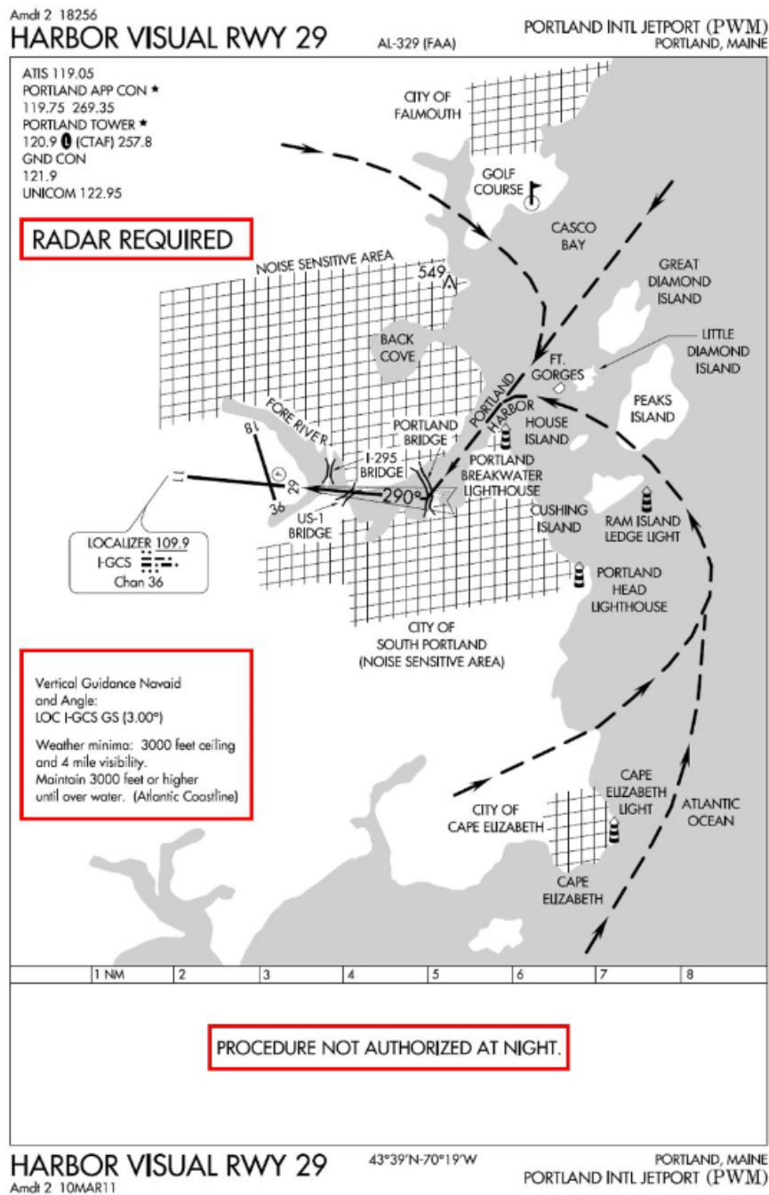
Figure 15.34. Charted Visual Flight Procedure.
