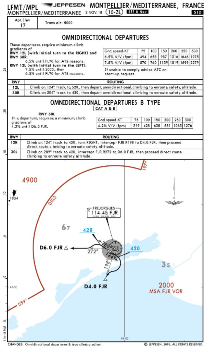
Figure 5.6. Omnidirectional Departure.
