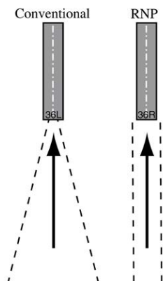
Figure 17.9. RNP Parallel Approach Operations.
