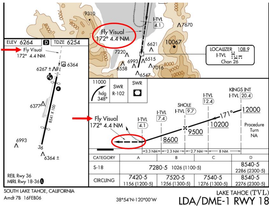
Figure 16.10. Visual Segment.
