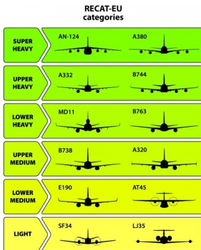
Figure 11.1. RECAT-EU Categories.
